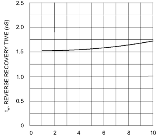
Fig. 4 Reverse Recovery Time vs. Forward Current
